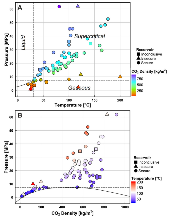
Fig. 4. CO 2 state diagrams of the studied naturally occurring CO 2 reservoirs. Dashed lines indicate critical pressure (7.38 MPa) and temperature (31 °C), the thick black line represents the vapour curve. (A) Pressure versus temperature plot highlights that reservoirs holding gaseous CO 2 are more likely to be insecure than reservoirs holding supercritical CO 2 . (B) Pressure versus CO 2 density plot illustrating that the majority of insecure reservoirs hold CO 2 with a low (<250 kg/m 3 ) density.
