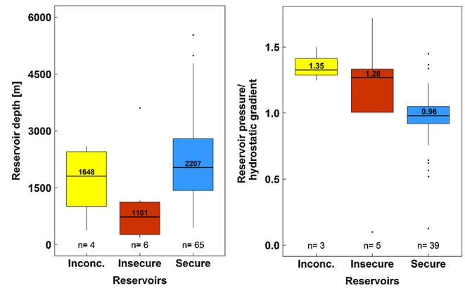
Fig. 3. Left: Boxplot of reservoir depth of naturally occurring CO 2 reservoirs against inconclusive (inconc.), insecure and secure reservoirs. Note that insecure reservoirs are mainly found in shallow depths (median of 1101 m) while secure reservoirs are generally deeper (2207 m). Right: Boxplot of reservoir pressure/hydrostatic gradient of naturally occurring CO 2 reservoirs against inconclusive (inconc.), insecure and secure reservoirs. Note that inconclusive and insecure reservoirs tend to be overpressured (reservoir pressure/hydrostatic gradient >1) while secure reservoirs show a wide range of pressures. The box plot shows the median (black horizontal line) and the interquartile range. The whiskers (black vertical line) depicts the 1.5 inter-quartile range.
