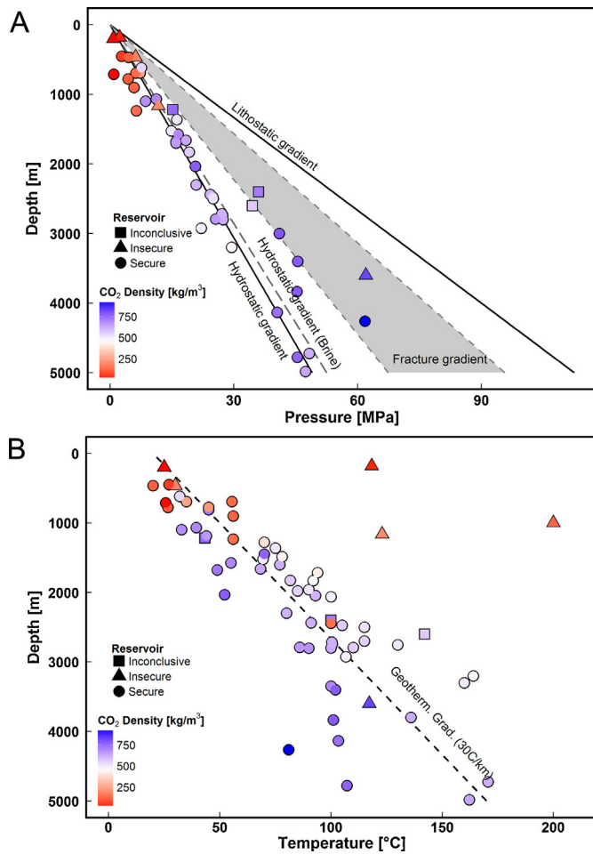
Fig. 2. (A) Depth versus pressure plot of naturally occurring CO 2 reservoirs with in situ pressure data. Note that insecure and inconclusive reservoirs are mainly shallow (<1200 m) or within the fracture gradient regime. Fracture gradients tend to range from 60 to 90% of lithostatic stress and depend on the sedimentary basin and tectonic regime. The deep, insecure reservoir with reservoir pressure in the fracture gradient regime is Pieve Santo Stefano, Italy (No. 36, SI Table 1). (B) Depth versus temperature plot of naturally occurring CO 2 reservoirs, based on in situ data. Note that a high geothermal gradient is associated with migration of CO 2 in shallow reservoirs.
