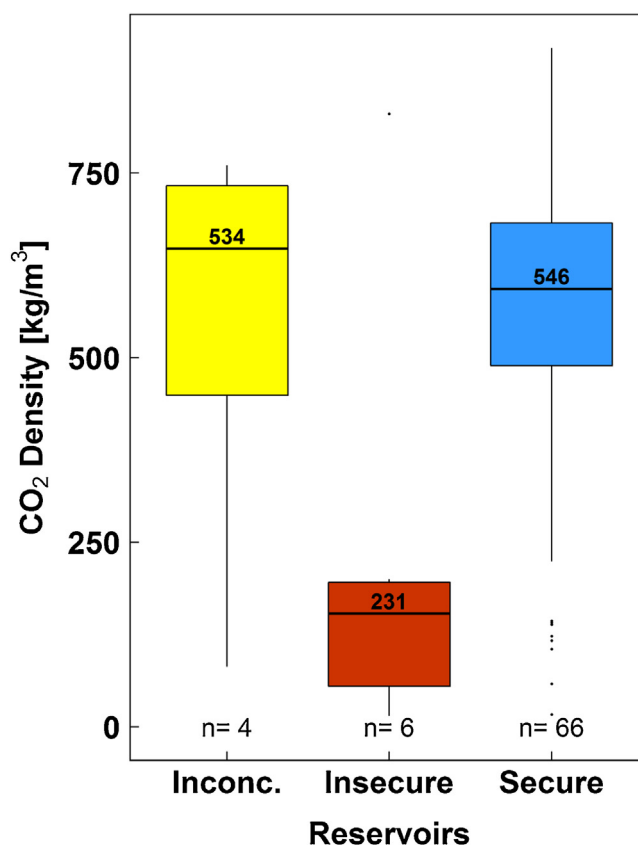
Fig. 5. Box plot of CO 2 density in naturally occurring CO 2 reservoirs against inconclusive (inconc.), insecure and secure reservoirs. Note that insecure reservoirs hold low density CO 2 (231 kg/m 3 ) while secure reservoirs on average have a higher density (546 kg/m 3 ). The box plot shows the median (black horizontal line) and the interquartile range. The whiskers (black vertical line) depicts the 1.5 inter-quartile range.
