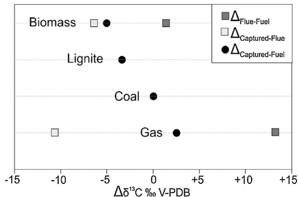
Fig. 3. Difference ( \Delta ) between average fuel, flue gas, and captured CO 2 \delta^{13}\text{C} values for fuel combustion with CO 2 amine capture.
