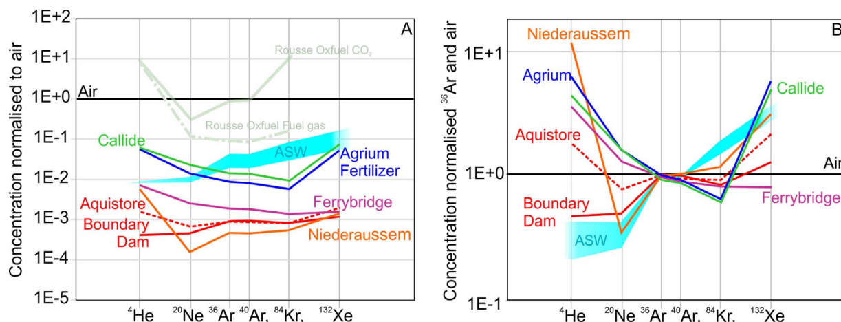
Fig. 6. Noble gas concentrations in capture \text{CO}_2 normalised to concentrations in air (A) and normalised to ^{36}\text{Ar} and air (B). Rouse data from Garcia et al. (2012). The range of air saturated water (ASW) noble gas concentrations for water equilibrated with air at between 10 and 60 °C (calculated according to Kipfer et al., 2002) is also shown. Ferrybridge = Sample Ferrybridge-2. All other samples are as described in Fig. 2. (For interpretation of the references to color in this figure legend, the reader is referred to the web version of this article.).
