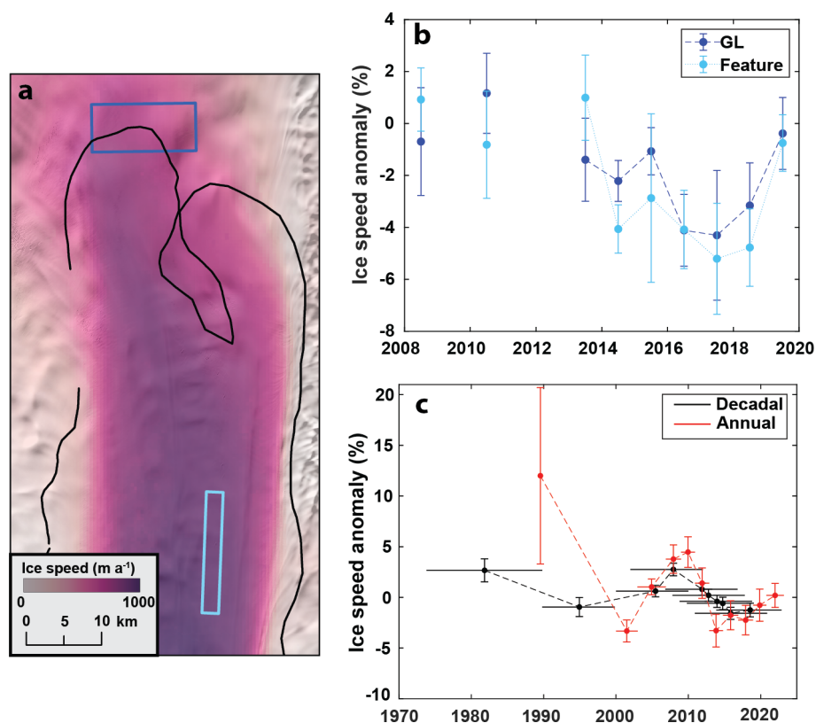
Figure 5. Ice-speed anomalies at Totten Ice Shelf. (a) Location of bounding boxes used to extract annual ice-speed anomalies at the grounding line (blue) and feature-tracking zone (light blue), with ice speed from the MEaSUREs ice velocity mosaic and grounding lines from October 2017 overlain (Floricioiu et al., 2021). (b) Annual ice-speed anomalies from the MEaSUREs annual mosaics. (c) Decadal and annual ice-speed anomalies extracted manually from within the feature box. Black data points represent decadal ice-speed anomalies; red data points represent the interannual ice-speed anomalies. Horizontal lines represent the time gap between the two images used to track surface features.
