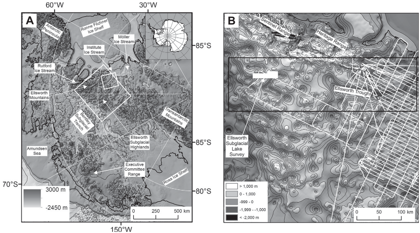
Figure 1. (A) Subglacial topography of West Antarctica (BEDMAP2) (m WGS84) (Fretwell et al., 2013), showing areas of Figures 1B, 6A–6C, 7A (large white box), and 3C (small white box). Inset shows location of study area. Thin black lines are bed topography contours at 1000 m intervals. (B) Subglacial topography of the Ellsworth Subglacial Highlands (BEDMAP2) (m WGS84) (Fretwell et al., 2013). Filled white polygons represent areas of exposed bedrock of the Sentinel and Heritage Ranges (from SCAR Antarctic Digital Database [ADD] ( http://www.add.scar.org/terms.jsp )). The white in-filled box delimits the area of the 2007–2009 ground-based RES survey of Ellsworth Subglacial Lake (Fig. 3A). Thick white lines show bed elevation measurements made during the 2010–2011 aerogeophysical survey of the Institute and Möller ice streams. Location of Figure 2 (large black rectangle) is shown. Thin black lines are bed topography contours at 250 m intervals.
