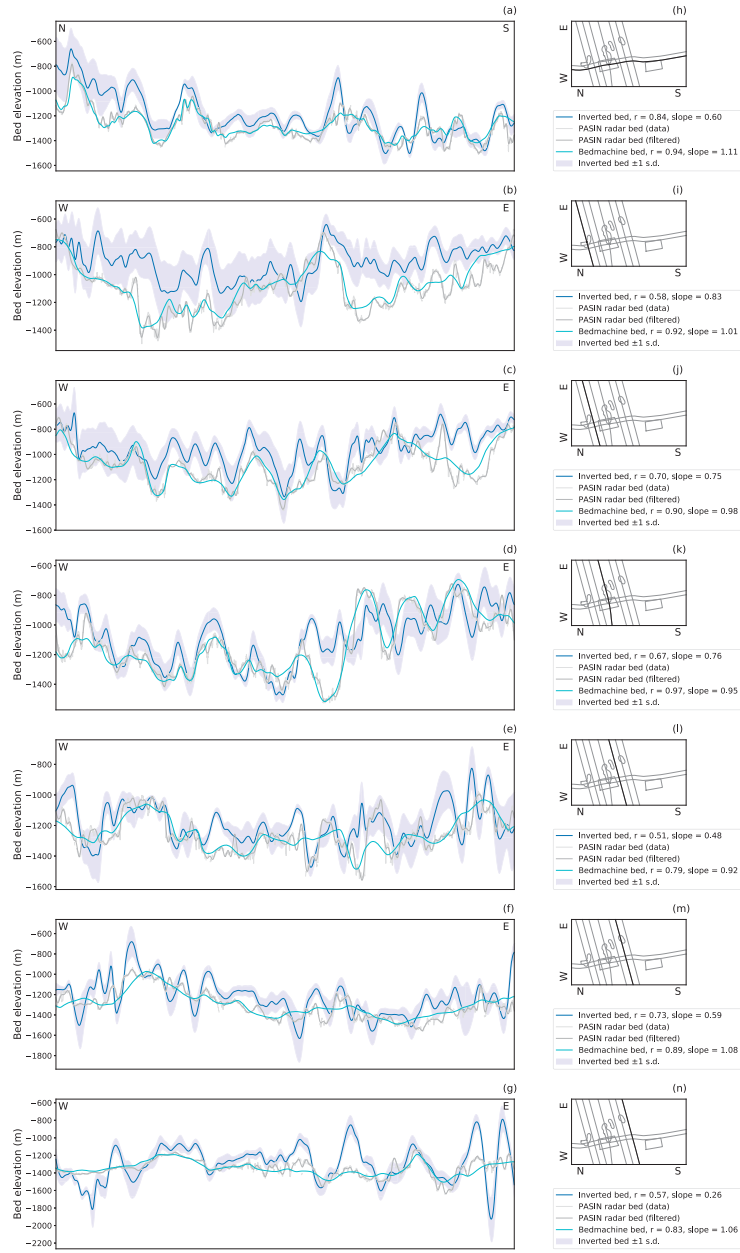
Figure S2. a) to g) Comparative plots of inverted bed topography with mean non-dimensional slipperiness \bar{C} = 100 with along flow radar-sounded bed topography. Bed topography is given as unfiltered bed picks from the 2019/20 airborne surveys; a version of the same filtered to 2 km wavelengths to be more representative of the detail we might expect to image in our inversion; and the bed profile extracted from BedMachine Antarctica (Morlighem et al., 2020). The envelope around the inverted bed topography shows plus or minus one standard deviation. The correlation coefficients ( r ) and slopes given are the results of a linear regression between the inverted bed or the BedMachine Antarctica bed and the filtered radar bed. h) to n) Profile locations within the inverted grid.
