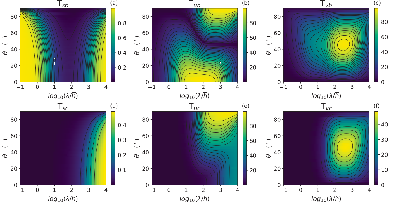
Figure S1. Panels (a), (b) and (c) show the non-dimensional shallow-ice-stream transfer functions T_{SB} , T_{UB} and T_{VB} between non-dimensional bed topography B and surface topography S ; along flow velocity U ; and across flow velocity V , respectively. Panels (d), (e) and (f) show the non-dimensional shallow-ice-stream transfer functions T_{SC} , T_{UC} and T_{VC} between non-dimensional bed slipperiness C and surface topography S ; along flow velocity U ; and across flow velocity V , respectively. All transfer functions are calculated for mean slipperiness \bar{C} = 100 , sliding law constant m = 1 , and mean surface slope \alpha = 0.002 . \theta is the angle of basal variability to the direction of flow, such that \theta = 0 for landforms aligned with the ice flow, and \theta = 90 for landforms perpendicular to the ice flow. \lambda is the wavelength of variability and is non-dimensionalised in terms of \bar{h} , the mean ice thickness, such that \log_{10}(\lambda/\bar{h}) = 1 means that \lambda = 10\bar{h} . T_{sb} = 0.1 means that variability in the surface topography will have one tenth of the amplitude of variability in the bed topography at that angle and wavelength. Similar figures can be seen in Gudmundsson (2008) with \bar{C} = 99 .
