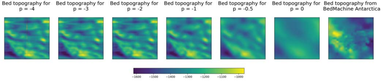
Figure S3. Bed topography results of the inversion for the Upper Thwaites region (see Figure 6 for location) with a variety of values of p_{filt} . Increasing p filters out increasing long wavelengths, and so a value of p_{filt} = -2 is chosen to filter out noisy short wavelengths, while maintaining realistic bed features, as compared to Bedmachine Antarctica (Morlighem et al., 2020).
