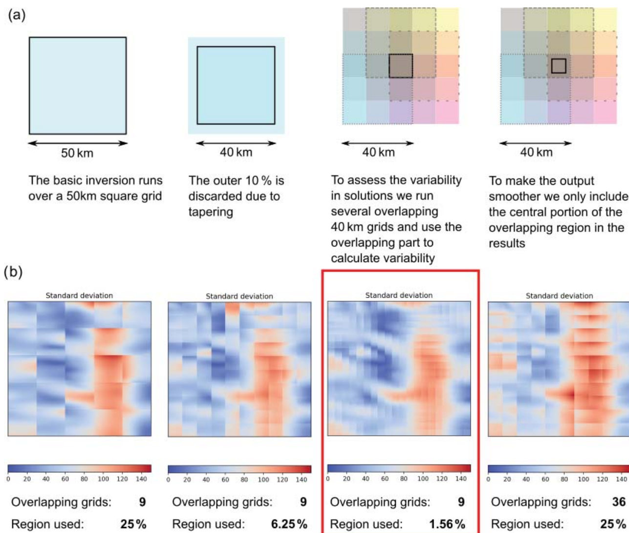
Figure 4. (a) Multiple overlapping grids are used in the inversion when applied to real data to allow the variability between solutions to be studied. (b) The effect of changing the number of overlapping grids and the fraction of the overlapping central region used to calculate the standard deviation of bed topography from the inversion in a roughly 60 km by 60 km region.
