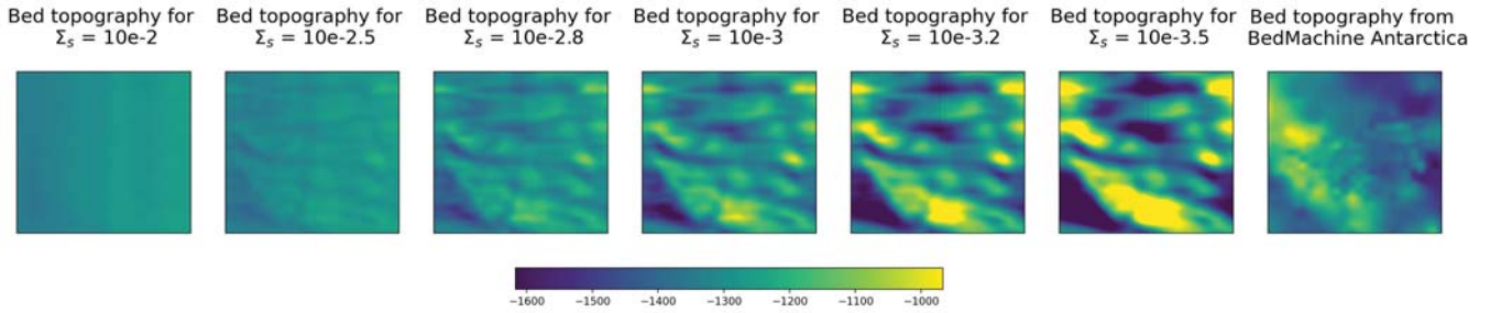
Figure S4. Bed topography results of the inversion for the Upper Thwaites region (see Figure 6 for location) with a variety of values of \Sigma_s . The weighting factor \Sigma_s controls the balance in the least squares inversion between the surface elevation and surface velocity data, with smaller values of \Sigma_s weighting the inversion towards the surface elevation. A value of \Sigma_s = 0.001 is chosen to produce realistic amplitude bed features, as compared to Bedmachine Antarctica (Morlighem et al., 2020).
