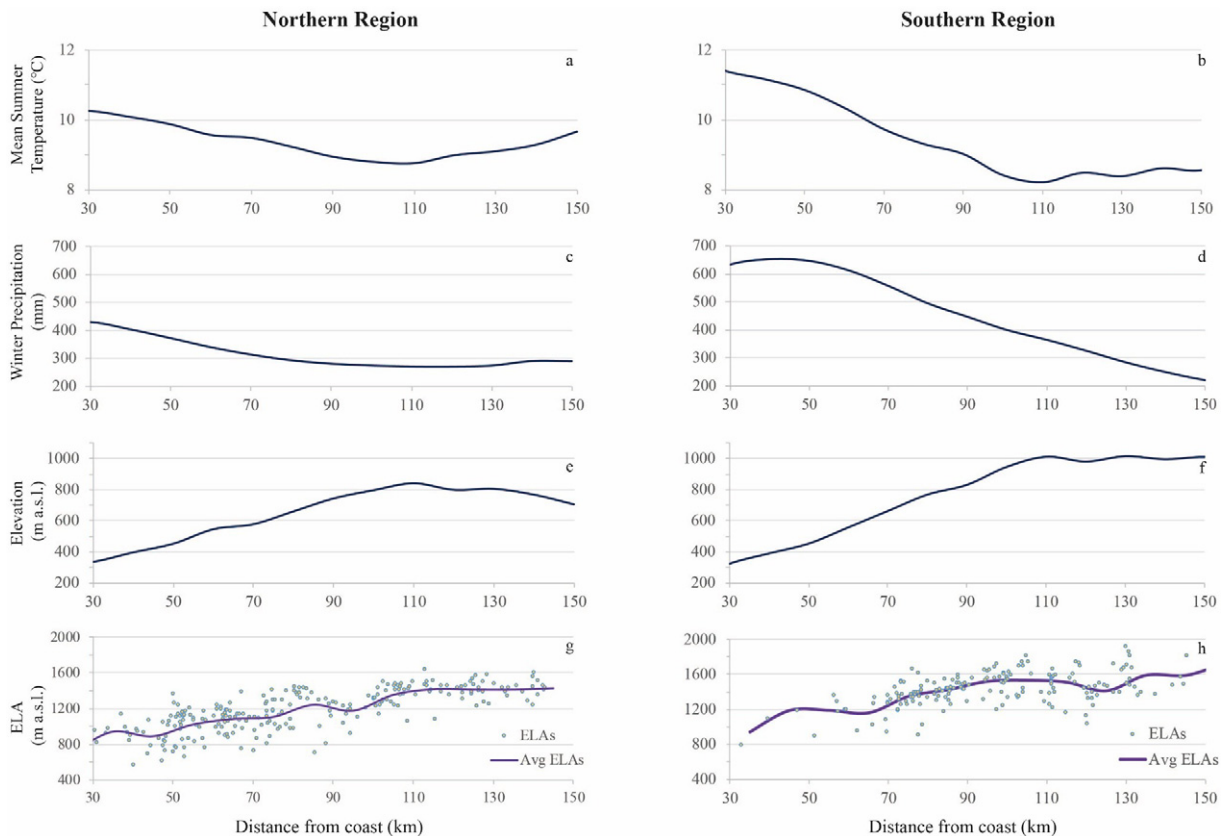
Fig. 6. The plots show various trends with distance from the coast extracted within 10-km wide swaths that were generated parallel to the coast in both the south and north Scandinavia macro-regions: (a) mean summer air temperature in the northern region; (b) mean summer air temperature in the southern region; (c) winter precipitation in the northern region; (d) winter precipitation in the southern region; (e) mean topography in the northern region; (f) mean topography in the southern region; (g) average ELA in the northern region overlain with individual cirque glacier ELAs (blue dots); and (h) mean ELA in the southern region with individual cirque glacier ELAs.
