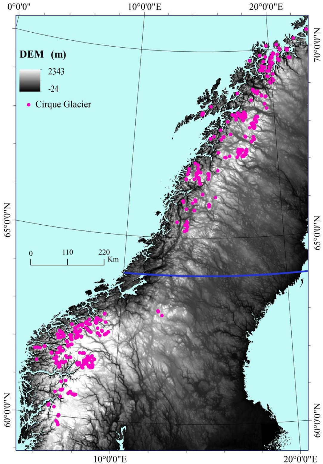
Fig. 1. Locations of cirque glaciers analysed within this study (pink dots). The topographic saddle at \sim 64^{\circ}\text{N} coincides with a latitudinal change in climatic zones. The thick blue line separates the two macro-regions discussed in the text.
