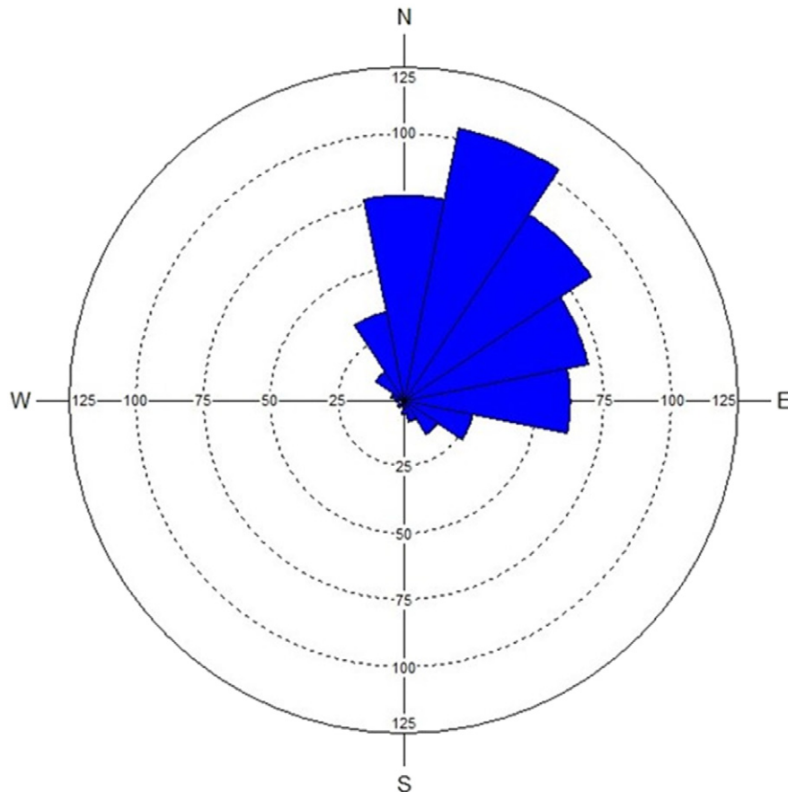
Fig. 7. Rose diagram of cirque glacier mean aspect ( n = 513 ). Each bin is 22.5^\circ , (i.e. North spans 348.75\text{--}11.25 ) and the radius is the quantity of cirque glaciers that fall within that aspect bin. The mean direction of all cirque glacier aspects is 41^\circ .
