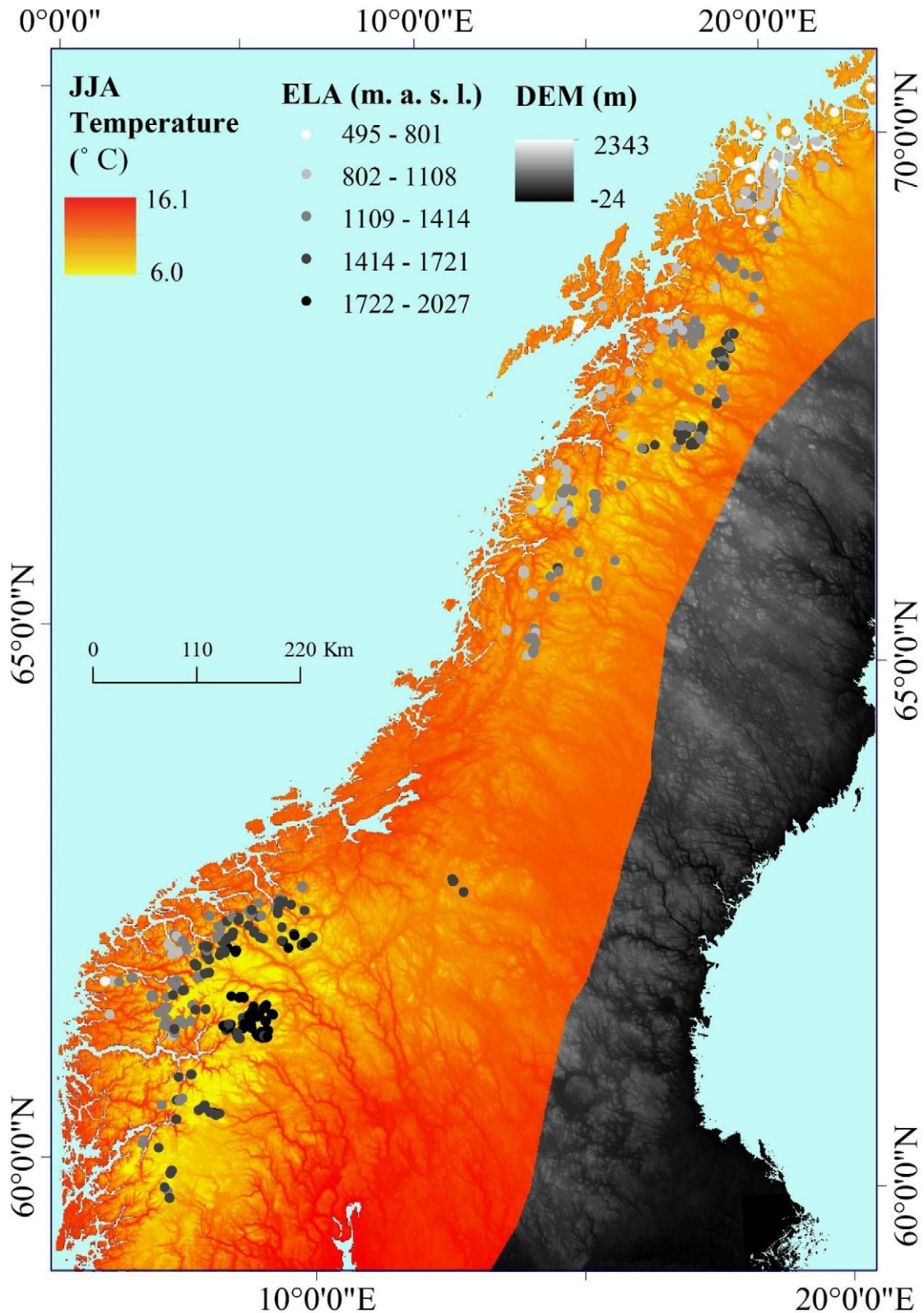
Fig. 3. Present day (1976–2006) mean summer temperature (JJA) across the study area. Modern cirque glacier ELAs are also shown. Climate data and DEM were obtained from the NVE (2017).
