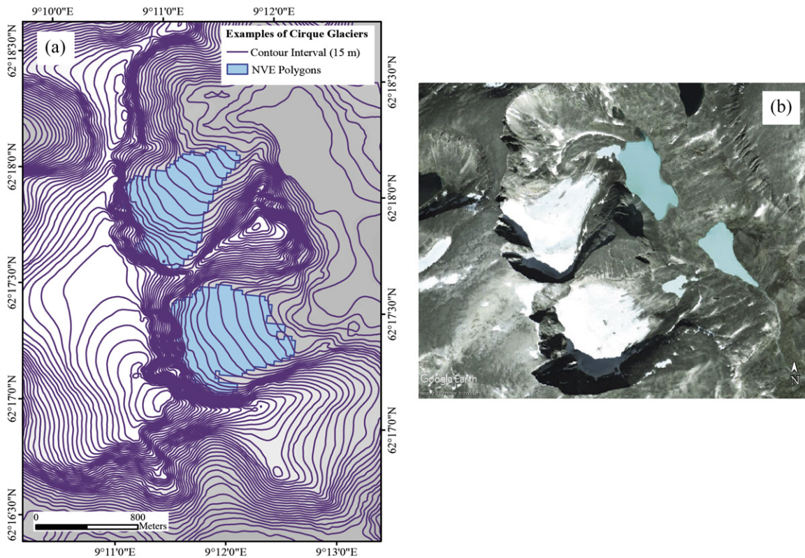
Fig. 2. Example of two cirque glaciers analysed in this study. (a) Cirque glacier polygons obtained from the NVE (2017). Also shown are 15 m elevation contours derived from the NVE DEM. (b) The same area viewed in a Google Earth image from the end of the ablation season in 2006, used to verify the presence of these glaciers. The top glacier is GLIMS ID G009186E62298N and the bottom glacier is GLIMS ID G009194E62289N located near the mountain Storstyggsvänätinden.
