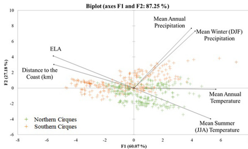
Fig. 5. PCA of potential controls on Scandinavian cirque glacier ELAs. The orange crosses are the southern cirque glaciers and the green are the northern cirque glaciers. Northern cirque glaciers are distributed along the temperature component. Southern cirque glaciers are distributed along two components, precipitation and distance to coast, both reflecting the effect of continentality on southern cirque glacier distributions.
