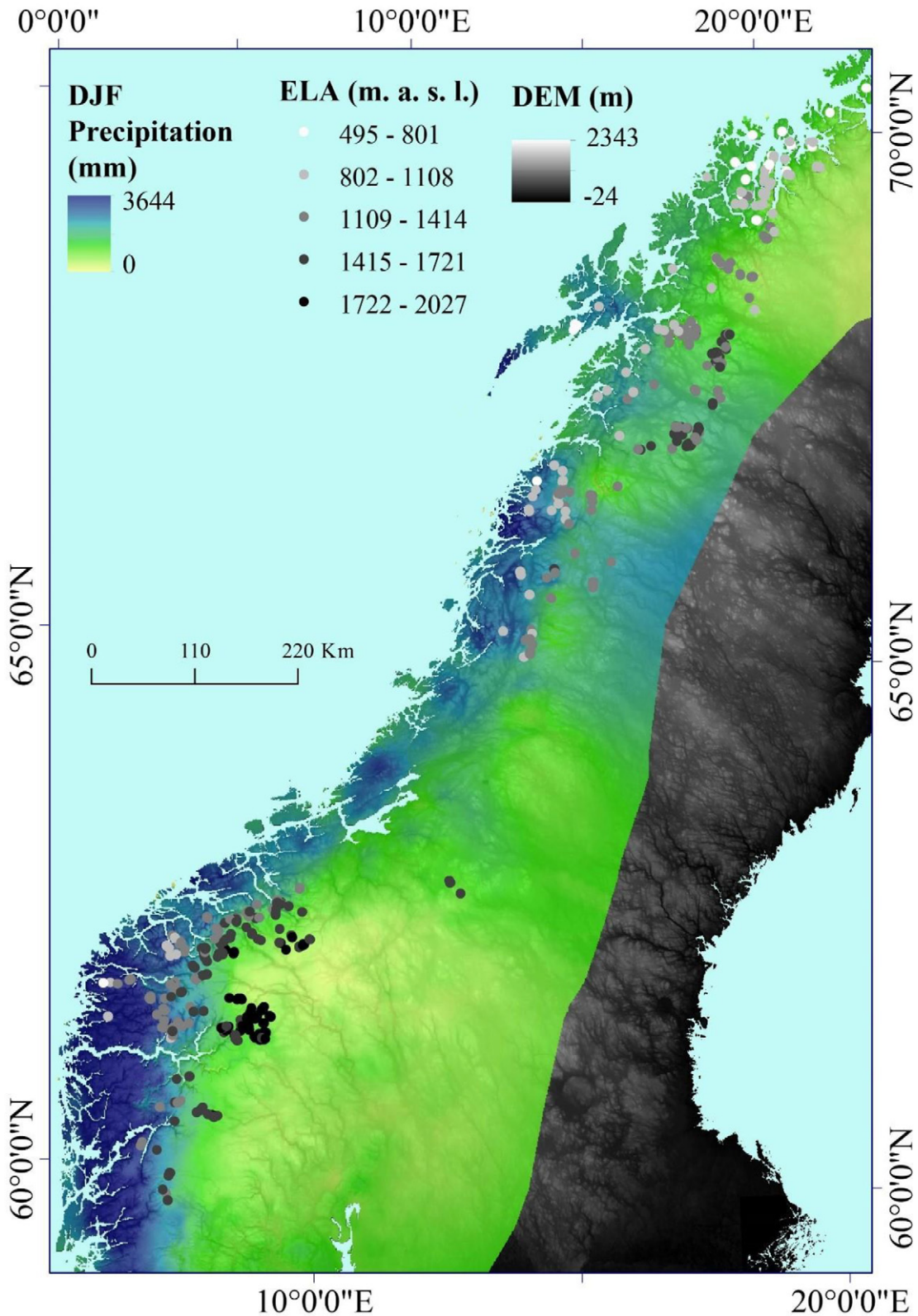
Fig. 4. Present day (1976–2006) winter precipitation across the study area. Modern cirque glacier ELAs are also shown. Climate data and DEM were obtained from the NVE (2017).
