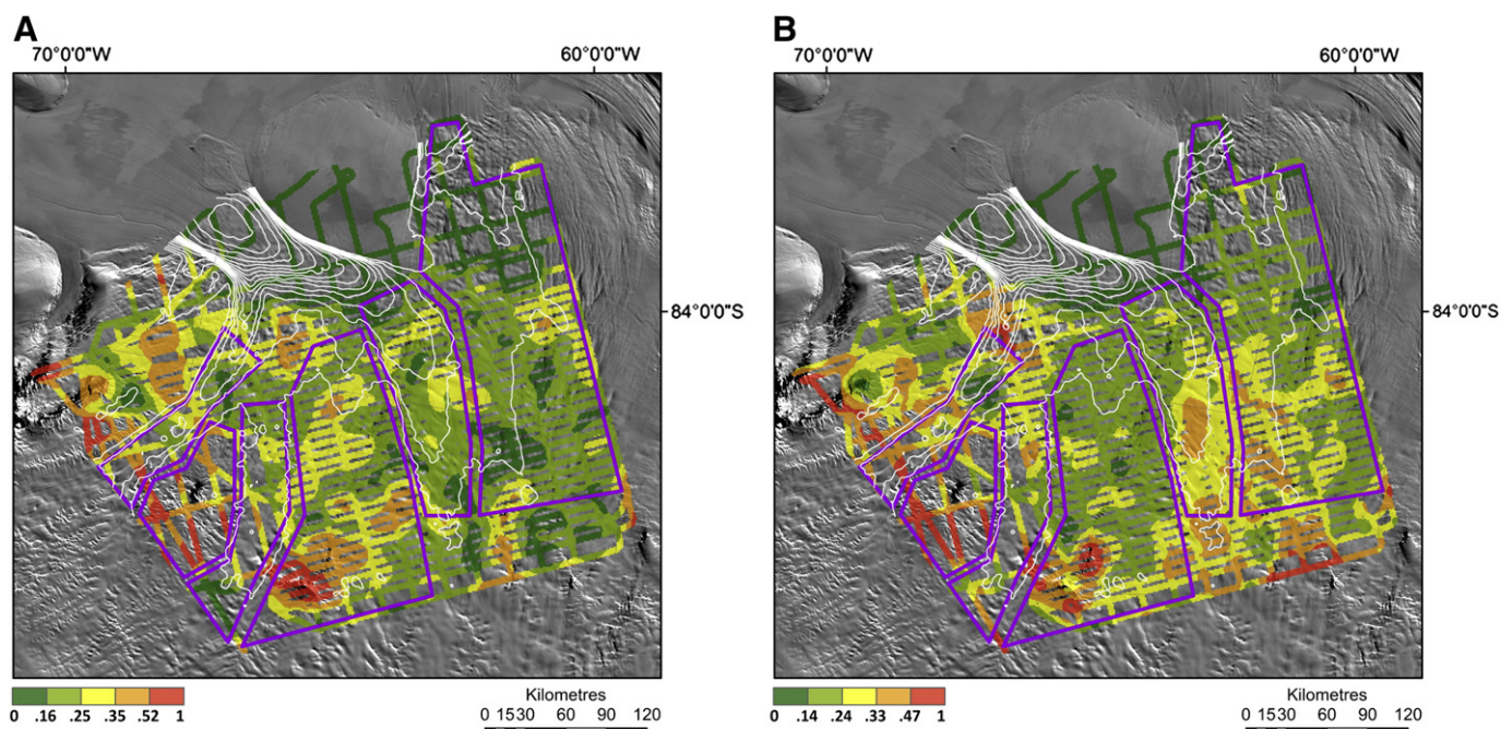
Fig. 5. Basal roughness determined using the standard deviation of along-track bed topography (A) parallel to flow and (B) orthogonal to flow. Roughness was calculated in both cases by identifying lines that were parallel or orthogonal to flow direction \pm 25^\circ (cf., Fig. 1B). Standard deviations were then calculated over a rectangular moving window over the terrain of 300 \times 300 m. These results were then interpolated onto a 1-km grid using the topo-to-raster routine in ArcGIS before being smoothed. Purple boxes delineate our previously defined zones (see Fig. 1A for an indicator of the naming conventions for each area).
