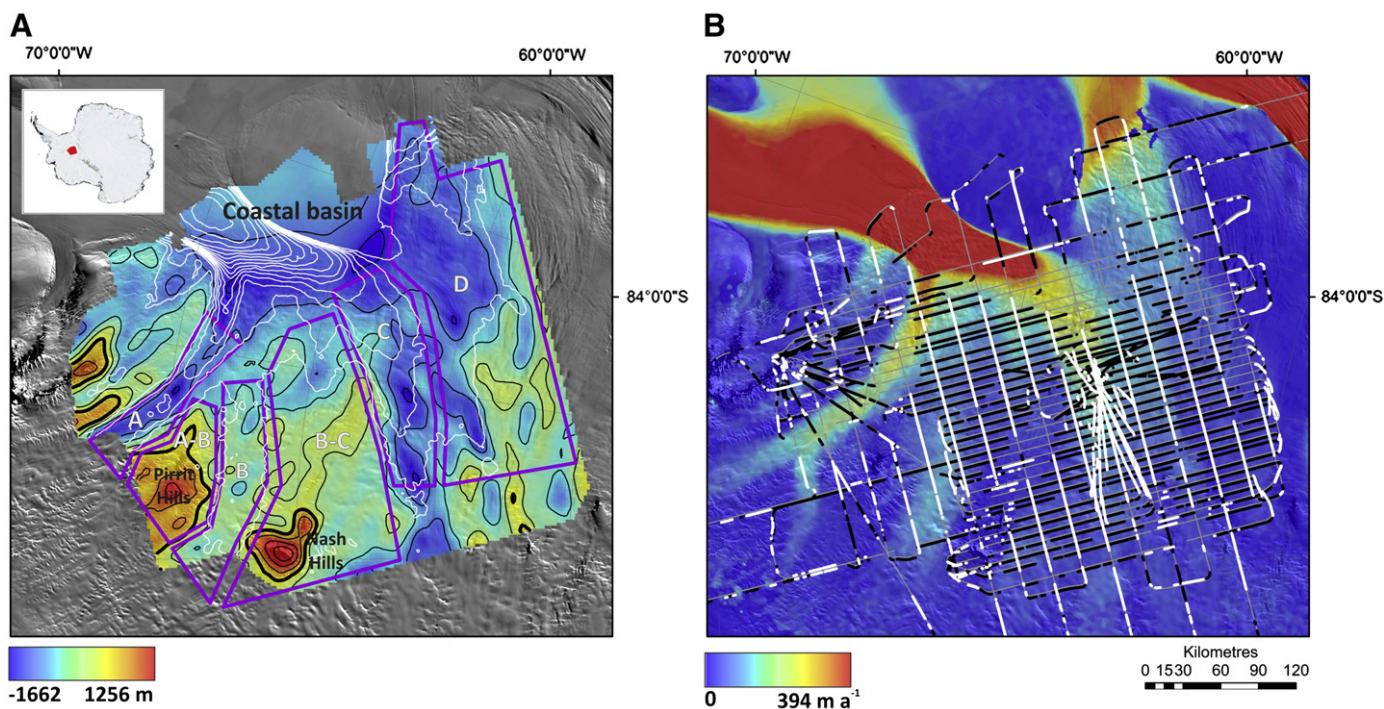
Fig. 1. Detailed maps of Institute and Möller Ice Streams in West Antarctica. (A) Background is a MODIS image with bed topography overlain in colour (and with thin black contour (400-m) lines) derived from our data (cf., Ross et al., 2012). The thick black contour represents current sea level. SAR-derived ice velocities (after Rignot et al., 2011) are visible as white contours ( 25 \text{ m a}^{-1} ) and clearly delineate the margins of IIS and MIS. Purple boxes outline the roughness subregions discussed later in the text. White letters within these boxes (areas A, B, C, and D) define regions incorporating tributaries of MIS and IIS; areas A–B and B–C are intertributary areas. The inset is a location map showing the study region in Antarctica. (B) Ice velocity (after Rignot et al., 2011) semitransparent over the MODIS image shown in (A). Overlying these are flightlines – the full data set is shown in grey, and lines are shaded white where they are parallel to flow and black where they are orthogonal to flow.
