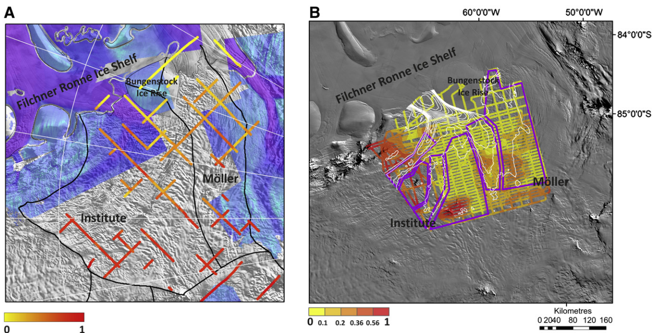
Fig. 3. Comparison of (A) original roughness map of IIS/MIS (adapted from Bingham and Siegert, 2007; their Fig. 1B) and (B) our new roughness estimates from high resolution data, degraded to an identical step size, and shaded using a similar colour scheme. Note that interpolation of roughness is limited to a 2.5-km buffer around flightlines. Purple boxes delineate our previously defined zones (see Fig. 1A for an indicator of the naming conventions for each area).
