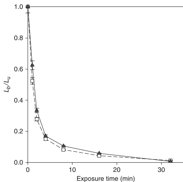
Fig. 8. Resetting of regenerated IRSL signals in samples 1285 (subglacial sediment; filled triangles) and 1296 (surface sediment) as a result of exposure to an artificial daylight source. The graph shows the observed signal after bleaching ( L_b ) as a proportion of the observed signal with no bleaching ( L_u ). Symbols are means of two aliquots per sample; errors were calculated as for Fig. 3.
