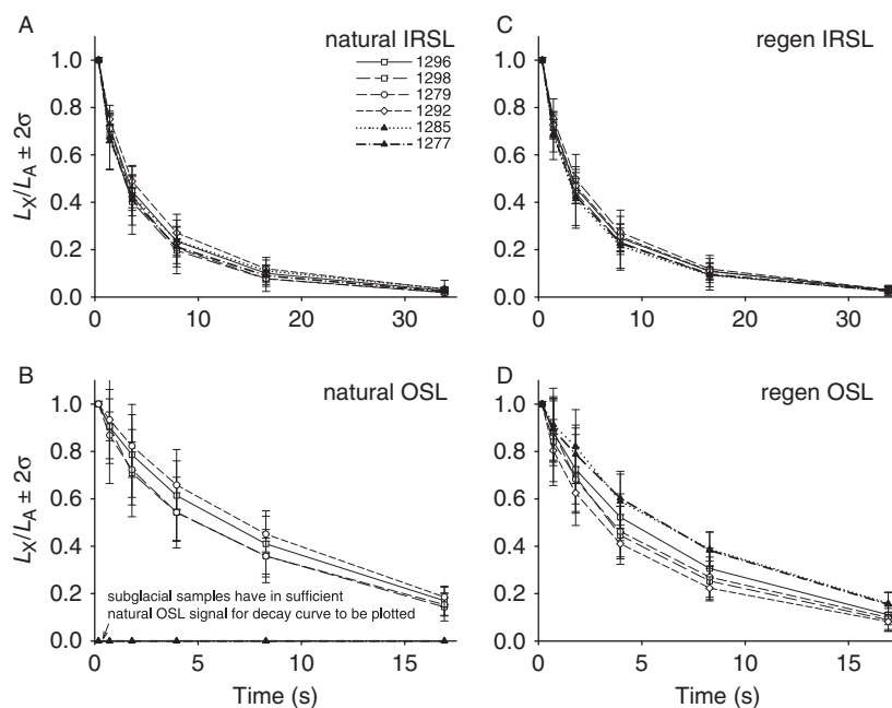
Fig. 6. Signal-decay plots obtained from IRSL and OSL shine-down curves for various samples: (A) natural IRSL; (B) natural OSL; (C) regenerated IRSL; and (D) regenerated OSL (key to all samples shown in (A)). The plots show sensitivity-corrected luminescence ( L_x ) for successive integration intervals (i.e. L_x = L_x/T_{x_s} , where x is the integration interval) as a proportion of the sensitivity-corrected initial signal ( L_A ) in interval a (integration intervals shown in Fig. 5). Values are means of eight aliquots per sample (except for 1279 in (A) and (B), for which values are means of seven determinations). Shine-down curves were measured using the multiple-stimulation approach of Table 1.
