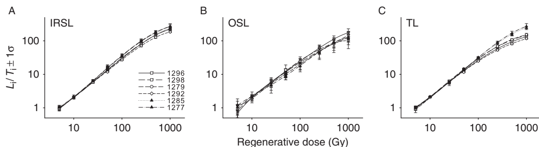
Fig. 4. Sensitivity-corrected luminescence growth-curves for various samples using a multiple-stimulation single-aliquot regenerative-dose (SAR) procedure (see text); regeneration points are means of eight aliquots per sample. All plots include a recycling point at 50 Gy; zero dose-point values (not shown) and recycling ratios are summarized in Table 4. Fitted curves are fourth-order polynomials that were also used to calculate the SAR D_e estimates (Table 3); for all curves R^2 > 0.999 and the standard deviation of the back-transformed residuals is < 3\% . The key to lines and symbols for all plots is shown in (A); see Fig. 1A for sample key.
