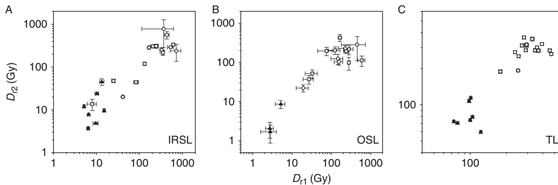
Fig. 3. Initial residual dose ( D_r ) estimates obtained using the simple polymineral single-aliquot multiple-stimulation screening procedure (see text). Two independent determinations of IRSL, OSL and TL D_r were obtained for each sample (i.e. D_{r1} and D_{r2} ) and these are shown on separate axes; error bars reflect photon counting statistics (Galbraith 2002) plus an estimated 2% analytical error (see Armitage et al. 2006). Subglacial samples are shown as filled triangles; see Fig. 1 for the key to other sample types. D_r values with errors that exceeded \pm 100\% , largely as a result of very weak L_n signals, were treated with caution; hence, one portal stream sample has been removed from (A) and six samples (including four subglacial sediment samples) have been removed from (B). See Supplementary Material for the full data set.
