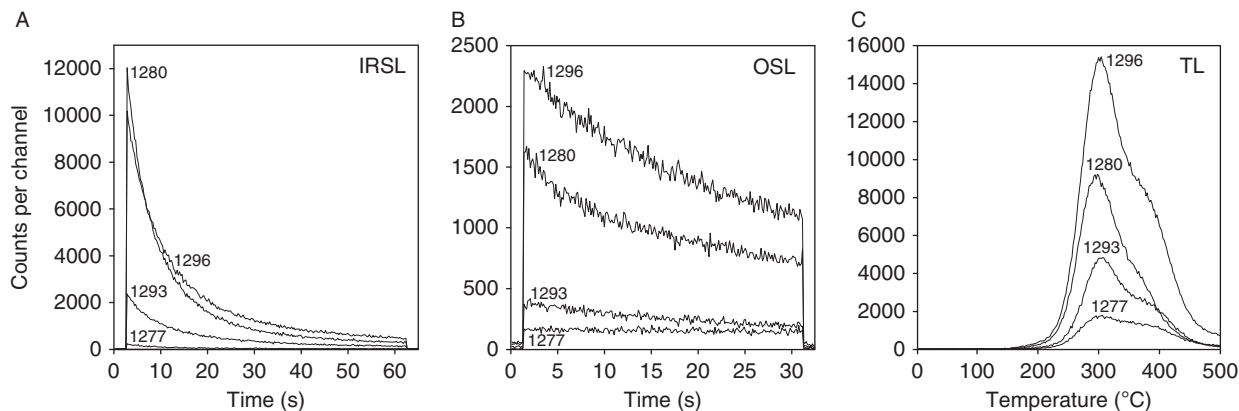
Fig. 2. Indicative IRSL and OSL shine-down curves and background-subtracted TL glow-curves measured during read-out of naturally trapped charge from individual discs prepared from samples 1277 (subglacial sediment), 1280 (portal stream sediment), 1293 (marginal stream sediment) and 1296 (surface sediment). IRSL and OSL signals were calculated by subtracting the underlying background (determined over the last 14.4 and 7.2 s of observed signal for IRSL and OSL, respectively) from the initial signal (obtained by integration over the first 4.8 and 2.4 s of observed signal for IRSL and OSL, respectively); TL signals were obtained by integration of the observed signal over the range 300 to 400°C.
