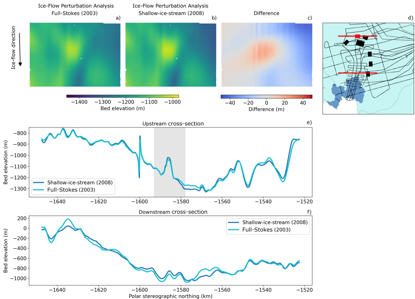
Figure 1. A comparison of bed topography produced from Ice-Flow Perturbation Analysis (IFPA) with the full-Stokes transfer functions from Gudmundsson (2003) and the shallow-ice-stream transfer functions from Gudmundsson (2008) for a 3D topographic patch (Site iSTART1), and two linear cross-sections. Mean non-dimensional slipperiness, \bar{C} = 100 . (d) Location figure marking patches of 3-D topography surveyed at high resolution with ice-penetrating radar in 2013/14 (Bingham and others (2017); black rectangles, with the patch in panels a–c coloured red), and airborne-radar profiles acquired in 2004/05 (Vaughan and others (2006); black lines, with red lines marking profiles in panels e and f). Panel (e) shows the comparison for the upstream cross-section, and panel (f) shows the comparison for the downstream cross-section. The grey highlighted section of panel (e) marks the profile's transition across Site iSTART1. Spikes at -1600 m in panel (e) result from an artefact of the transition between tiles of the REMA data, which could be avoided by using a continuous surface elevation product.
