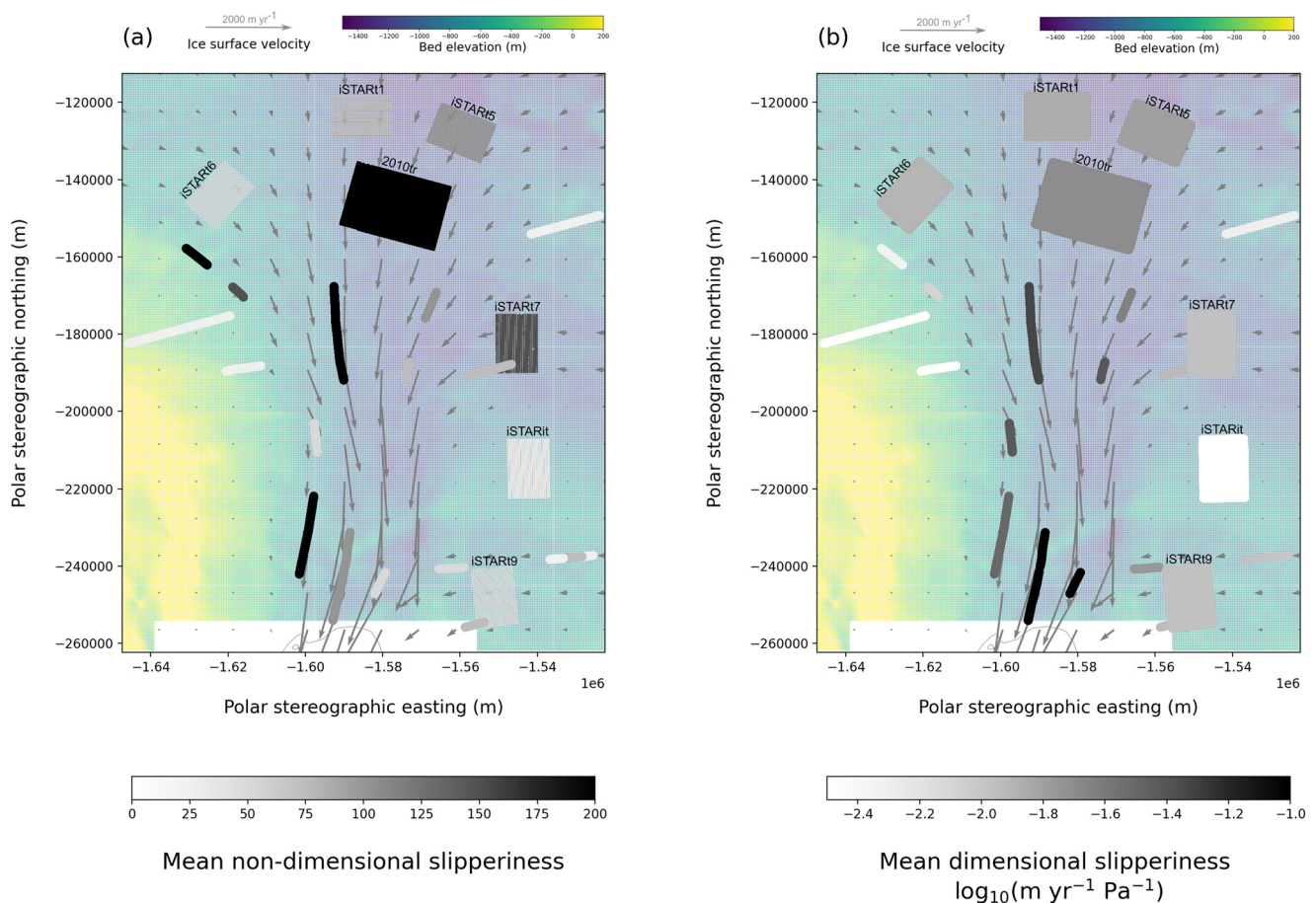
Figure 5. The best-fit mean slipperiness across Pine Island Glacier, as calculated by comparing the amplitude of landforms observed in radar measurements to those from IFPA, with bed topography and ice-surface velocity shown in the background. Both the airborne radar lines and ice-penetrating radar grids are shown. (a) Non-dimensional slipperiness, (b) dimensional slipperiness (note that this mostly varies with velocity). Higher slipperiness is observed in the main trunk and tributaries. Due to the mathematical inability of IFPA to resolve landforms aligned to flow ( k=0 ), only radar lines aligned to flow (which cross landforms at an angle to flow) have been used.
