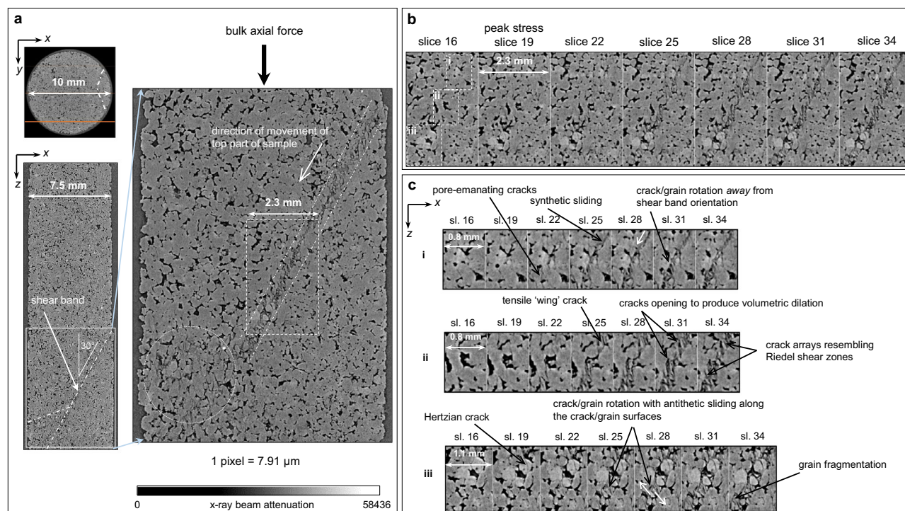
Fig. 2 | Microscale damage evolution close to and following peak stress.
