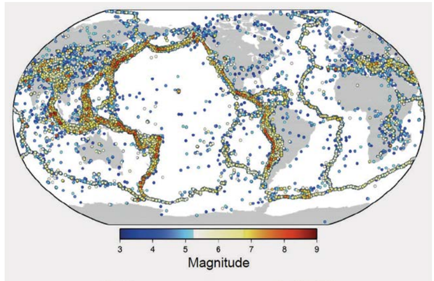
2 Global magnitudes and seismicity from the ISC-EHB catalogue.
