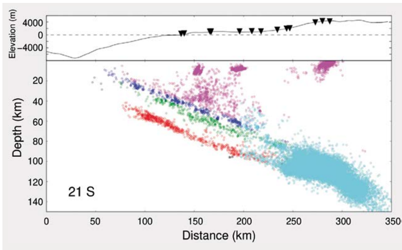
6 Cross-section through the Chilean subduction zone taken at 21°S with relocated seismicity superimposed. Magenta = upper plate events; blue = plate interface events; green = upper plane events; red = lower plane events; cyan = intermediate-depth cluster. Black triangles show seismometer positions on the ground surface. (Modified from Sippl et al. 2018)
